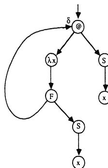
FIG. 6. Cyclic lambda graph corresponding to \delta = (\lambda x.F(\delta, Sx))(Sx) .
