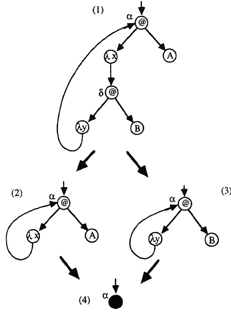
FIG. 9. Reductions to black hole.
